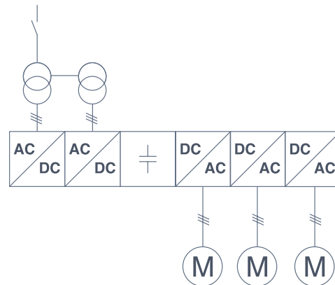
Diagram of common DC bus principle
