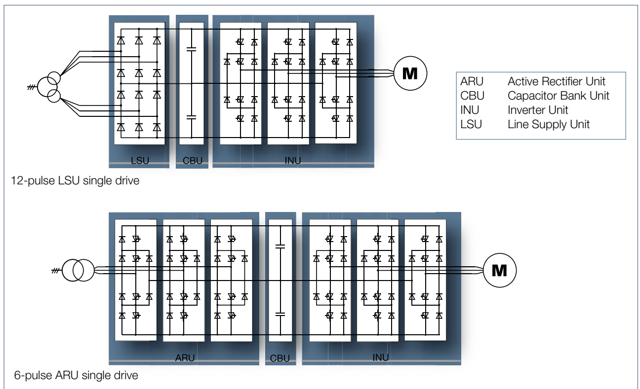
The ACS 6000 inverter topology
