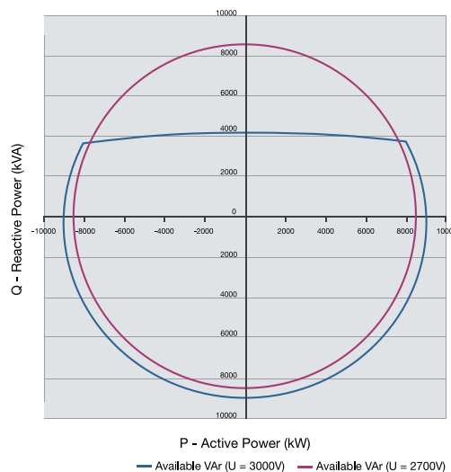
Diagram showing the available active and reactive power of the ARU
